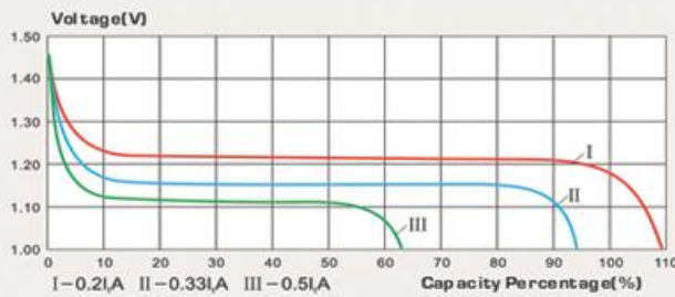
Figure 2 Discharging Curves of KPL Series ( 20^{\circ}\text{C} \pm 5^{\circ}\text{C} )
