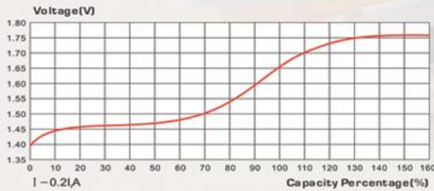
Figure 1 Charging Curves of KPL Series ( 20^{\circ}\text{C} \pm 5^{\circ}\text{C} )
