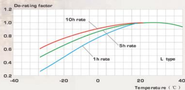
Figure 4 Temperature Effect Curves of KPL Series
